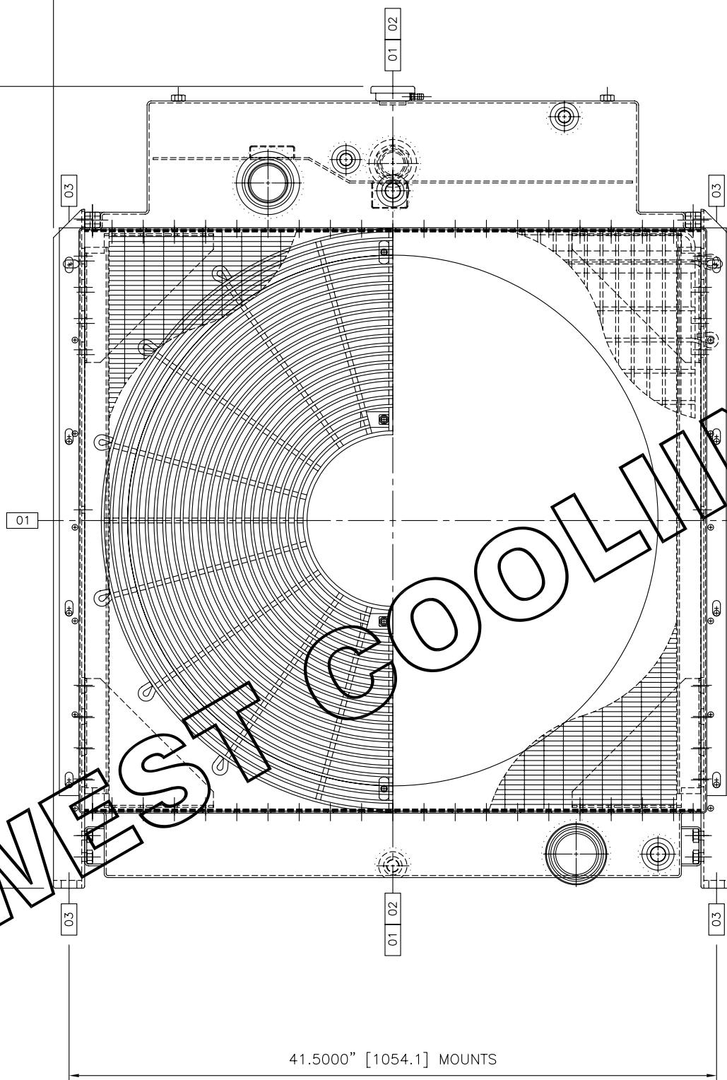
FRONT (FAN SIDE) ELEVATION
